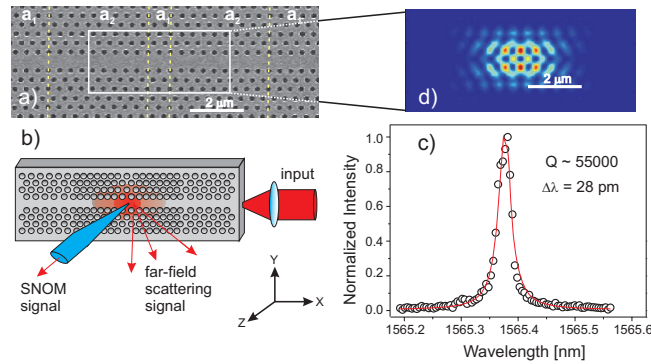
Fig. 1. Scanning electron micrograph of the heterostructure. The yellow lines mark regions with different lattice constants. a_1=410 nm, a_2 = 400 nm. (b) Schematics of the experimental arrangement. (c) The unperturbed cavity resonance as measured in the far field. The red curve is a Lorentzian fit to the measured data (black circles). (d) The calculated (FDTD) intensity distribution on resonance in the region marked by the white rectangle in Fig. (a).
